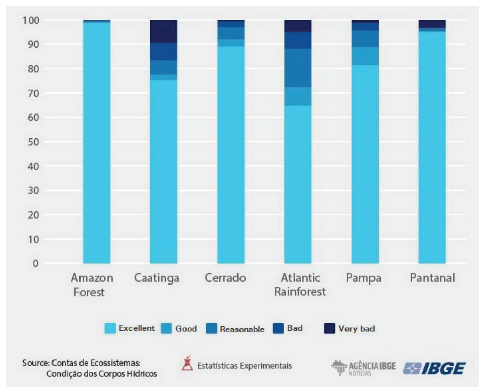
Figure 4: Capacity of water bodies to dissolve pollutants (2016) by biome.
